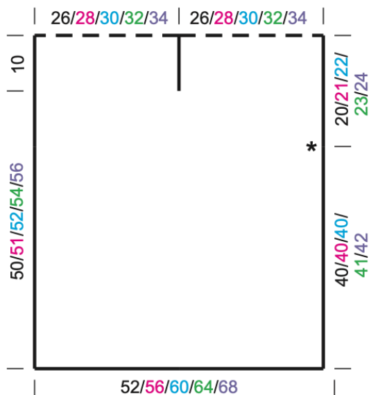
BACK PANEL
